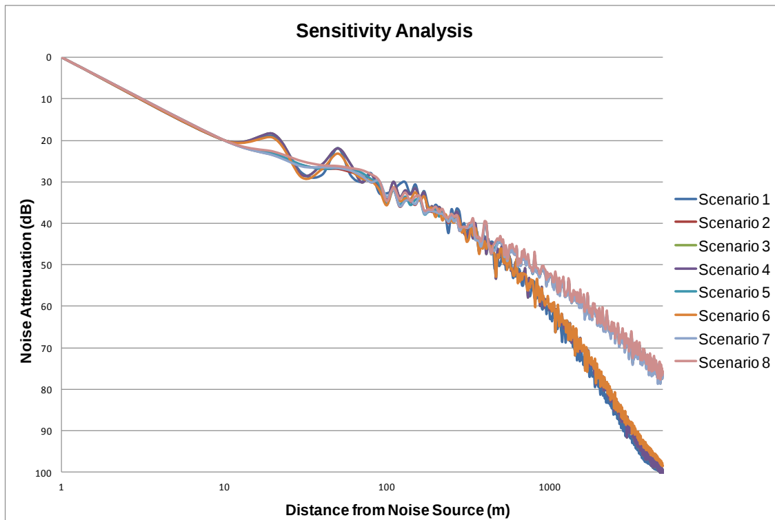
Figure 7.1: Sensitivity Analysis
