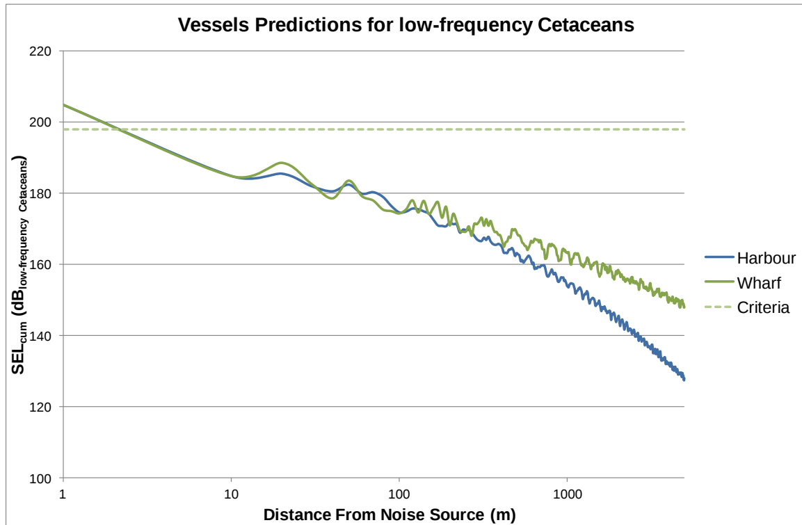
Figure D.1: Vessel Noise Predictions for low-frequency Cetaceans
