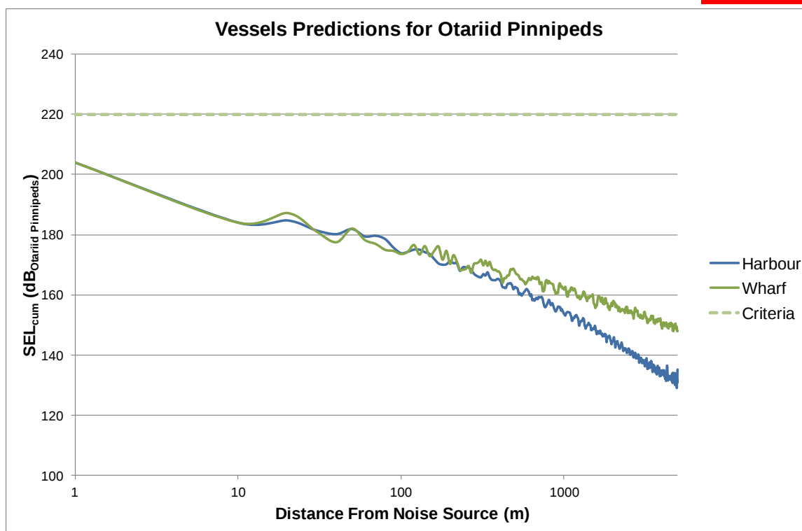
Figure D.3: Vessel Noise Predictions for Otariid Pinnipeds
