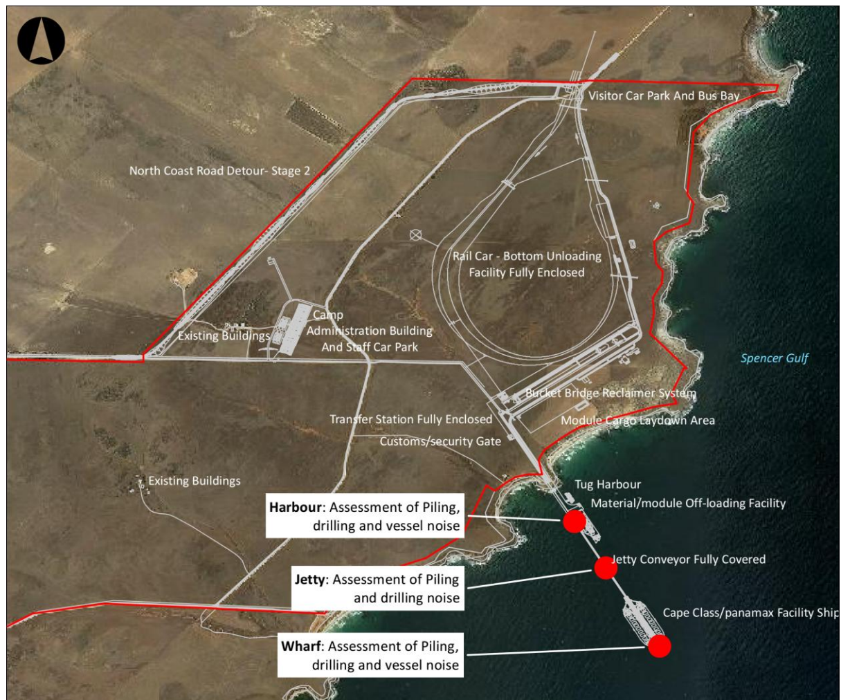
Figure 7.2: Noise Source Locations
