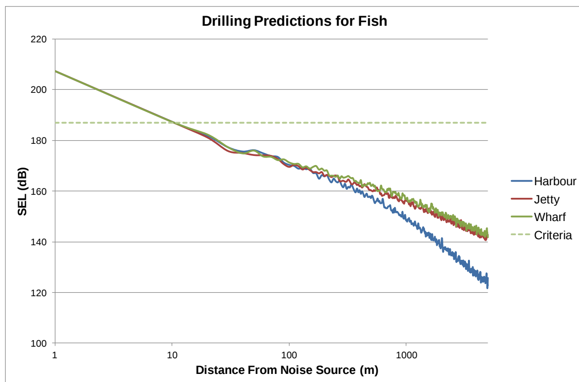
Figure C.4: Drilling Noise Predictions for Fish
