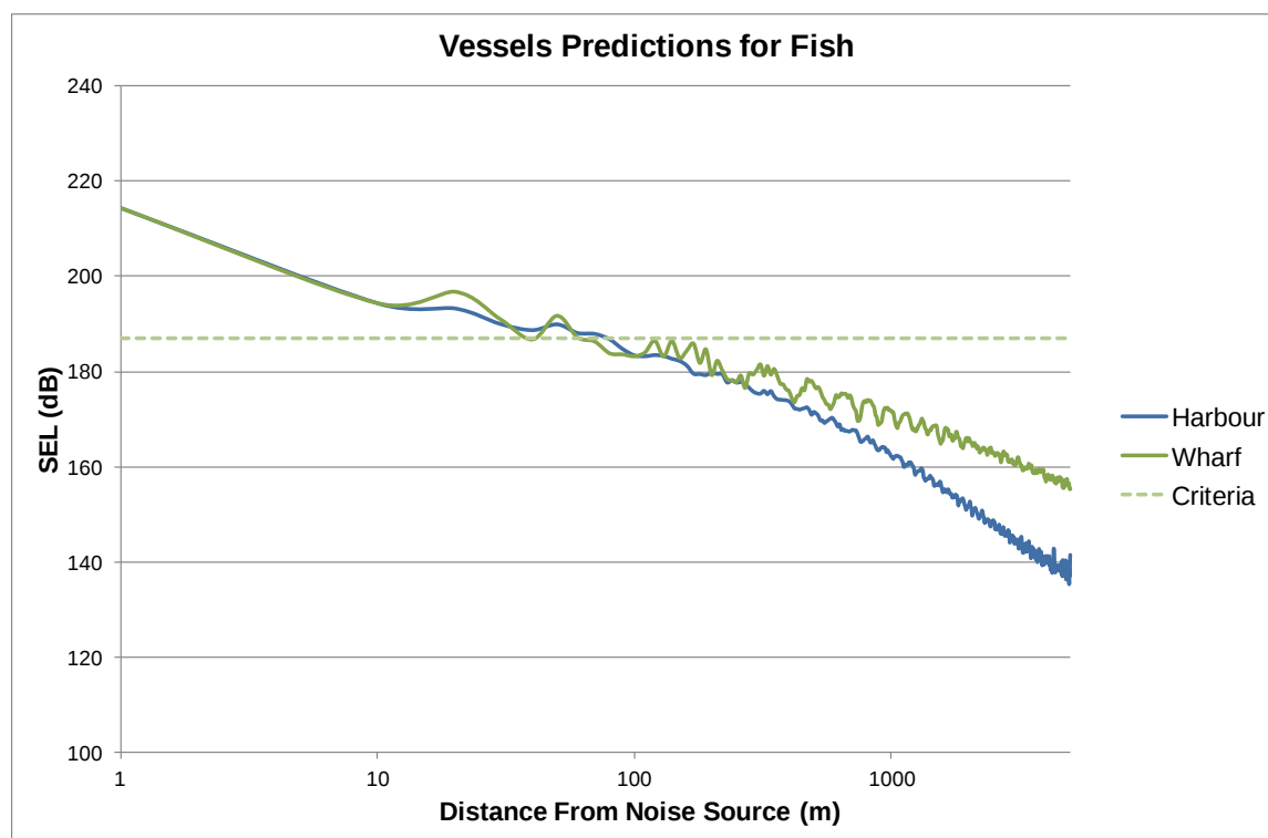
Figure D.4: Vessel Noise Predictions for Fish
