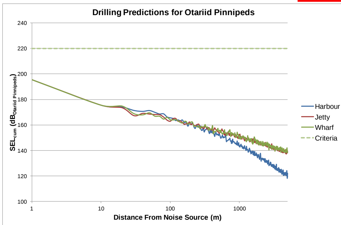
Figure C.3: Drilling Noise Predictions for Otariid Pinnipeds
