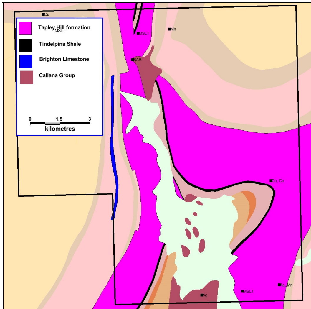
Figure 3: Geology Map for EL909 (PIRSA)
