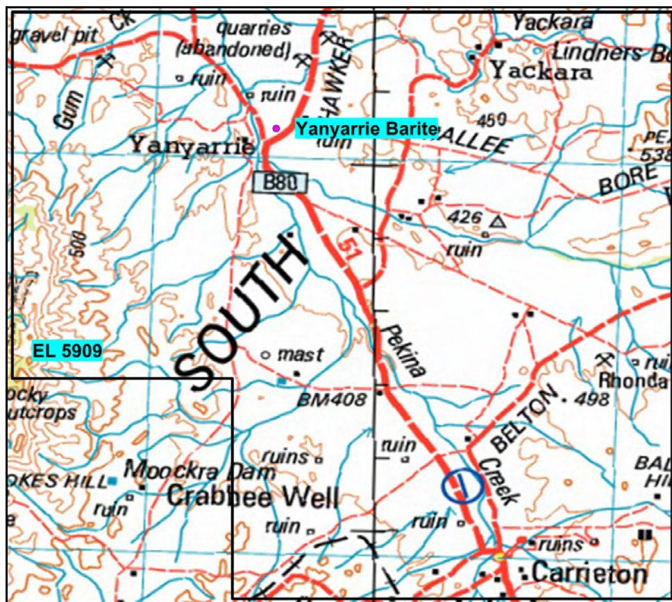
Figure 1: Location Map EL 5909, with Yanyarrie barite shown.
