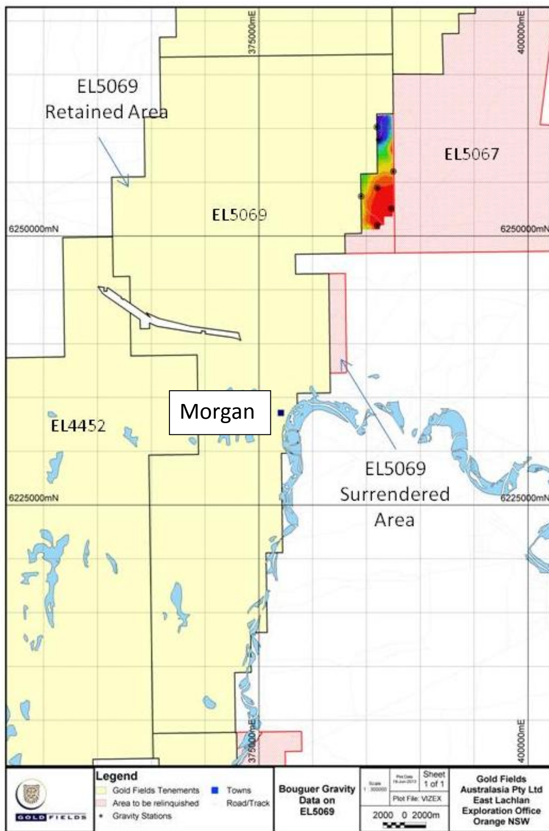
Figure 3: Ground Gravity completed on Relinquished area of EL5069.
