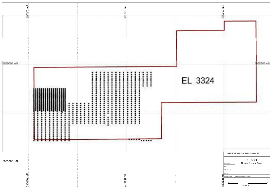
Figure 2 EL 3324 Gravity Station Locations.
