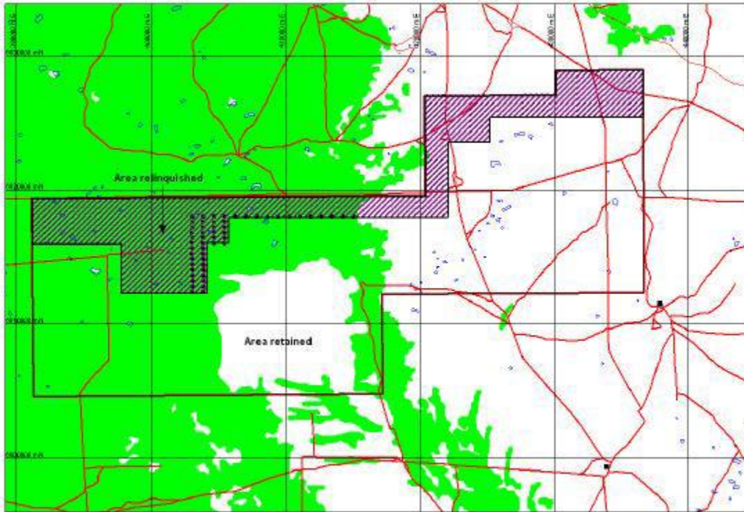
Figure 4: EL 3324 Gravity station locations on relinquished area
